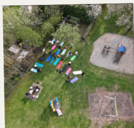
1. Training
